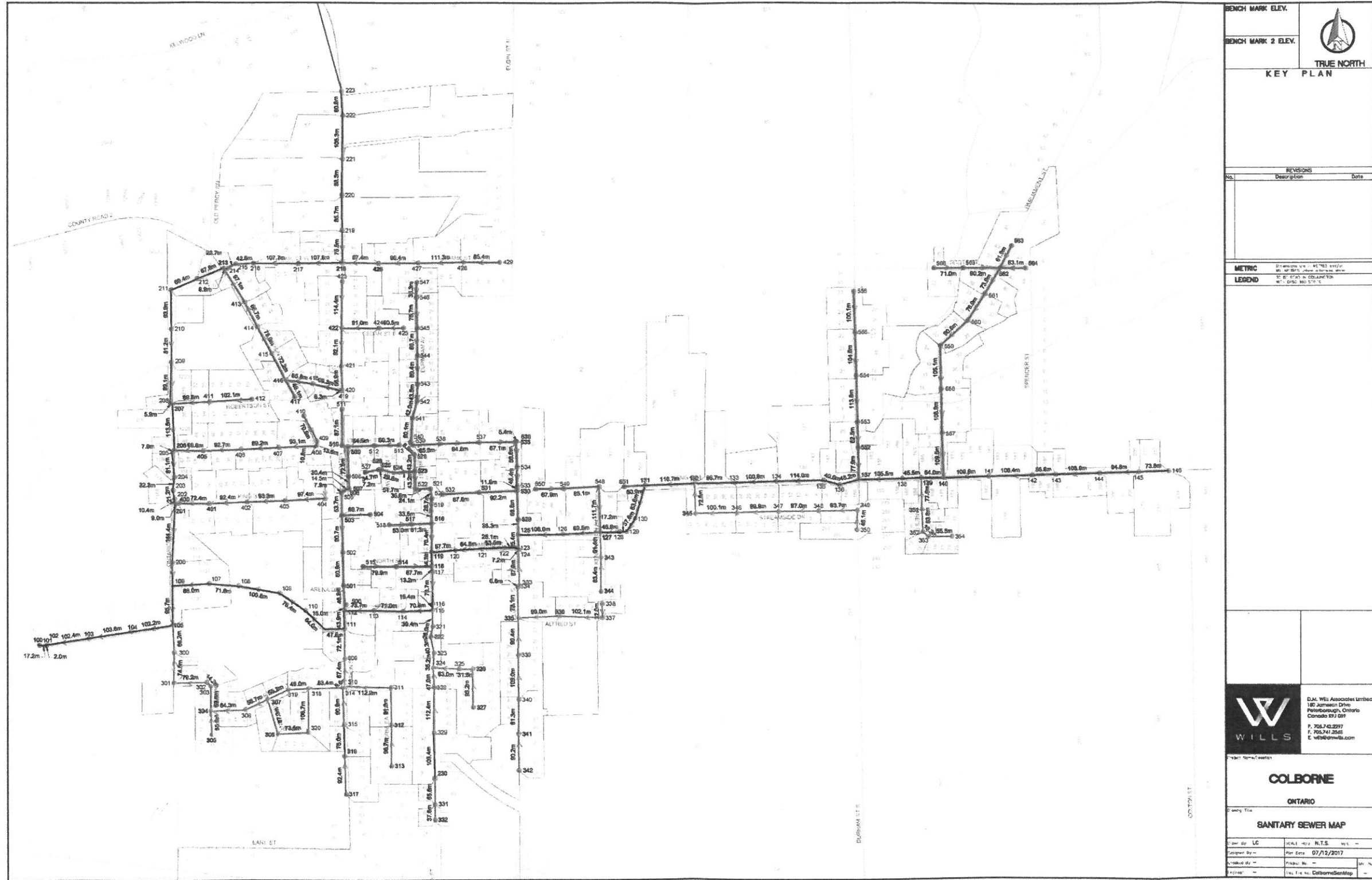
Figure 7 – Existing Colborne Sanitary Collection Network
